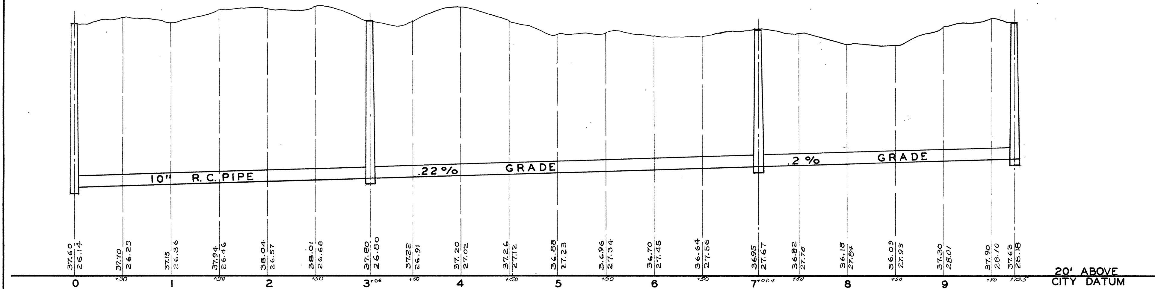
PLAN AND PROFILE OF BILLINGS PARK SECOND POINT SEWER
