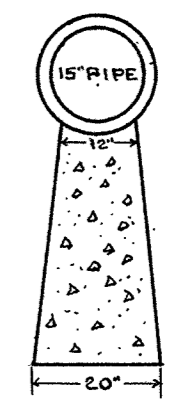
CROSS SECTION OF SUPPORTING WALL STA 222+82 TO STA 223+40
