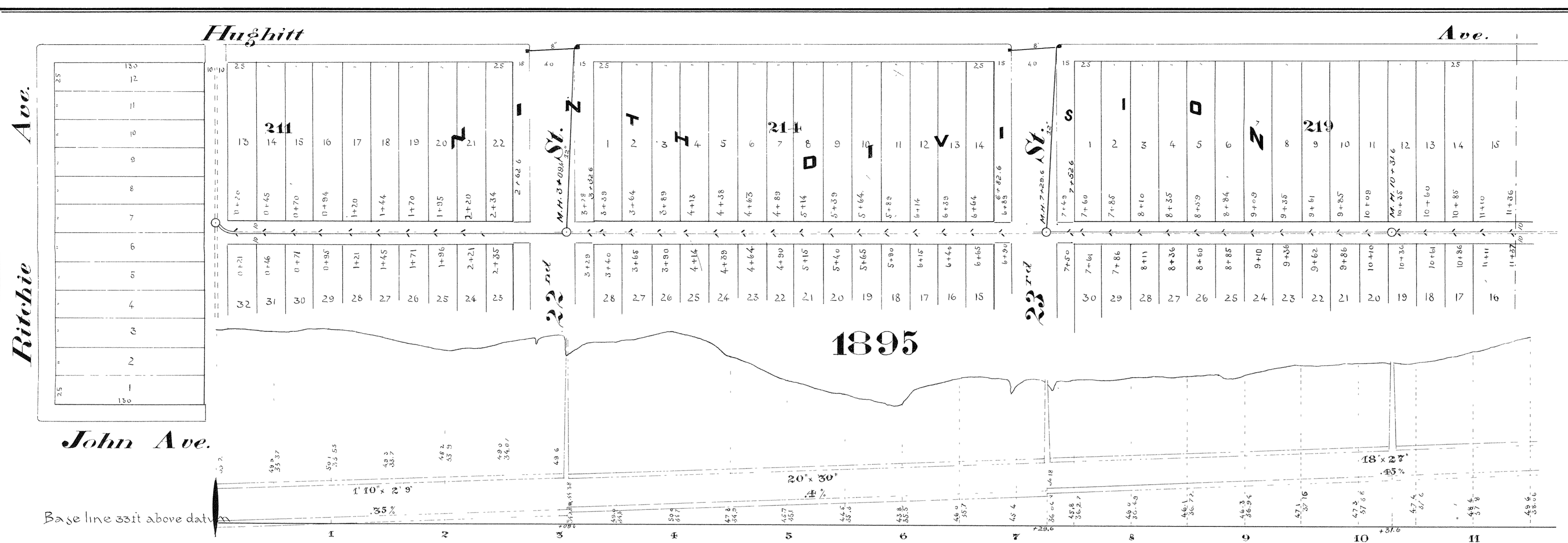
Plan & Profile of Sewer in Alley between John & Hughitt Aves. from Ritchie to Billings Ave.
