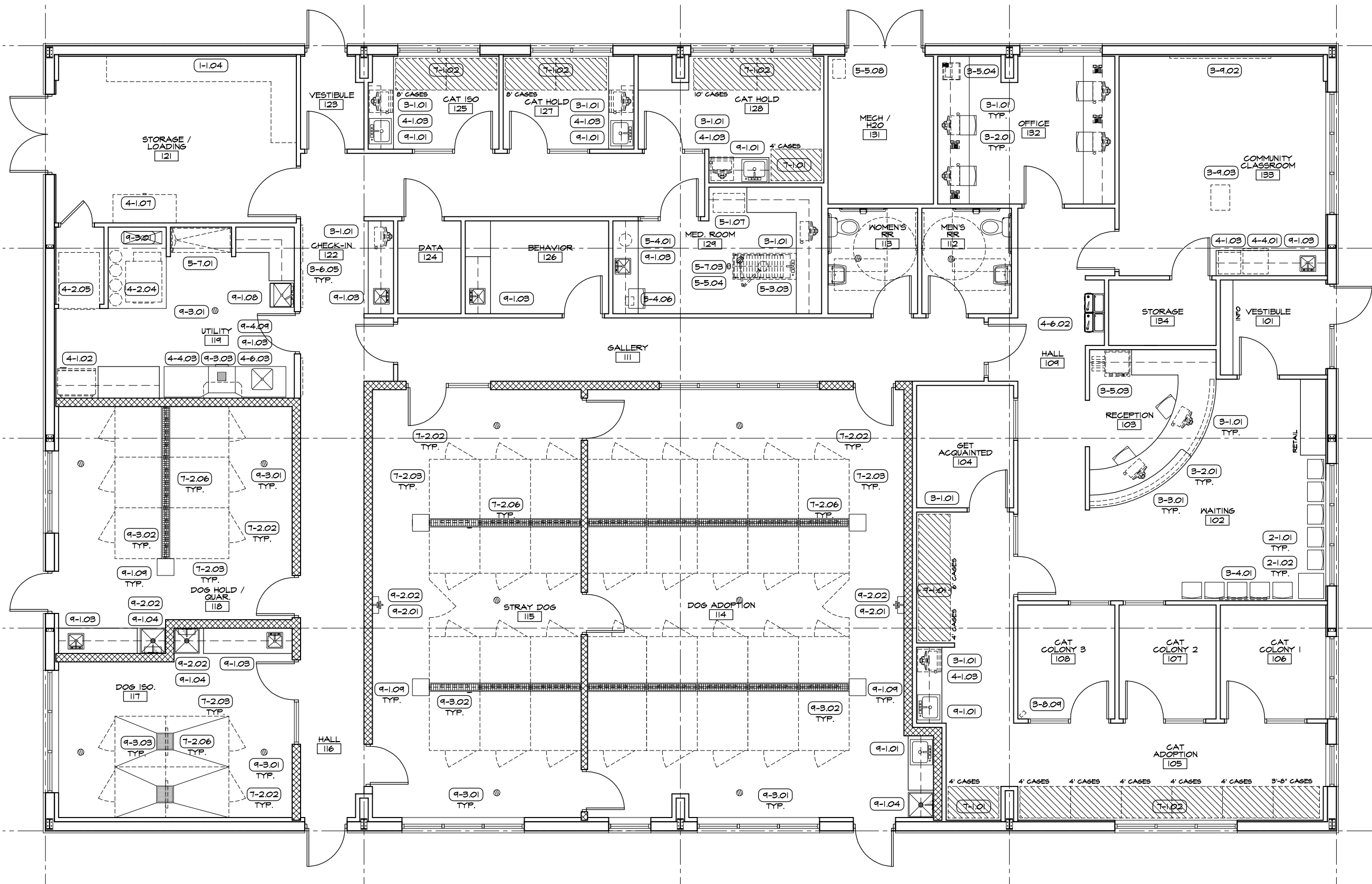
2 EQUIPMENT PLAN SCALE: 1/8" = 1'-0"
