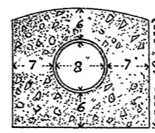
SECTION OF SEWER IN CONCRETE
