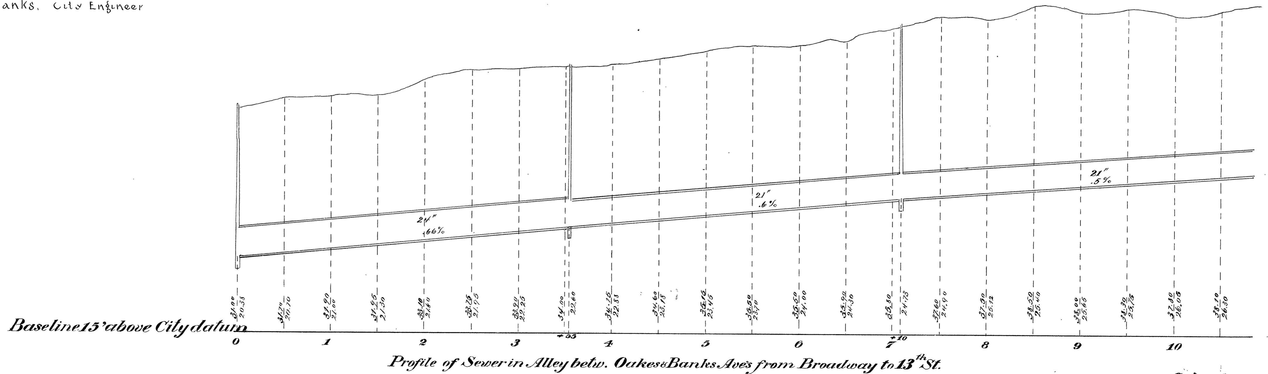
Section of 21 inch pipe
