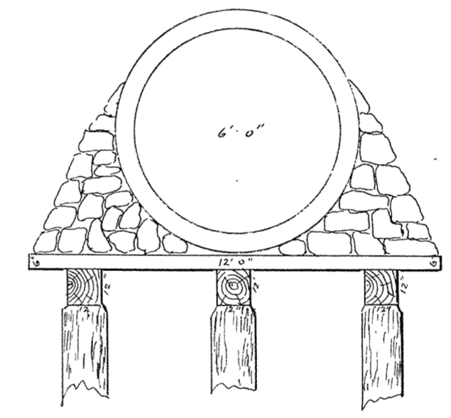
Section of 6' Sewer on Pile
