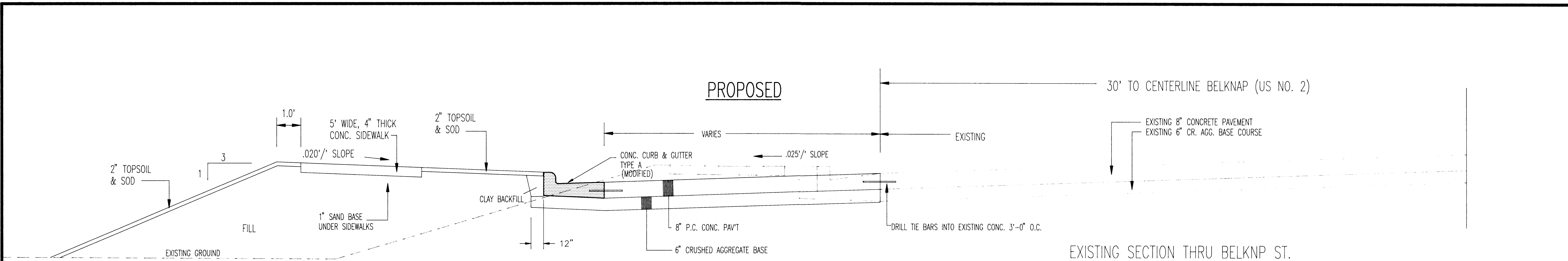
TYPICAL FINISHED SECTION FOR BELKNAP STREET (US NO. 2)
