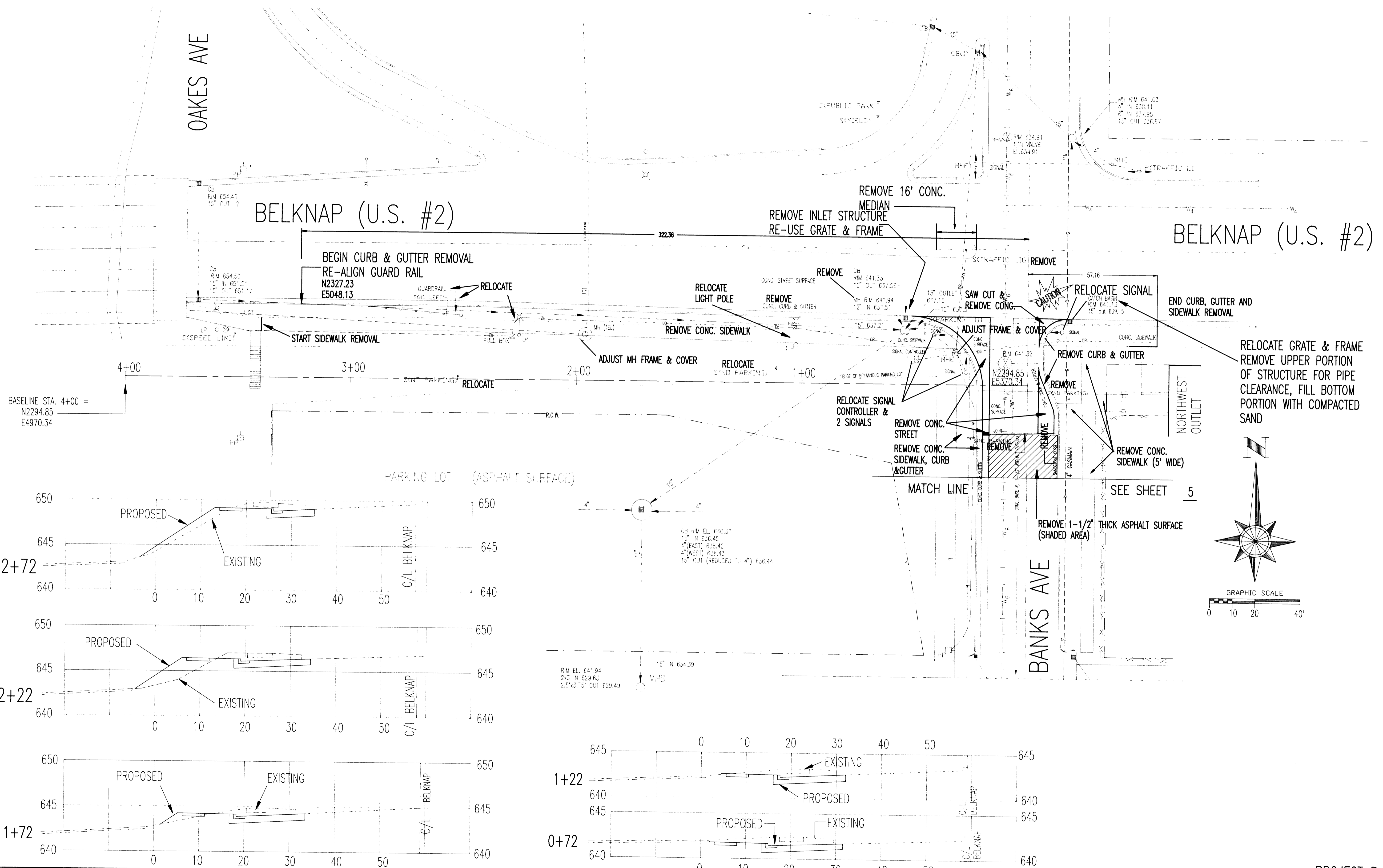
EXISTING TOPOGRAPHY AND REMOVAL PLAN
