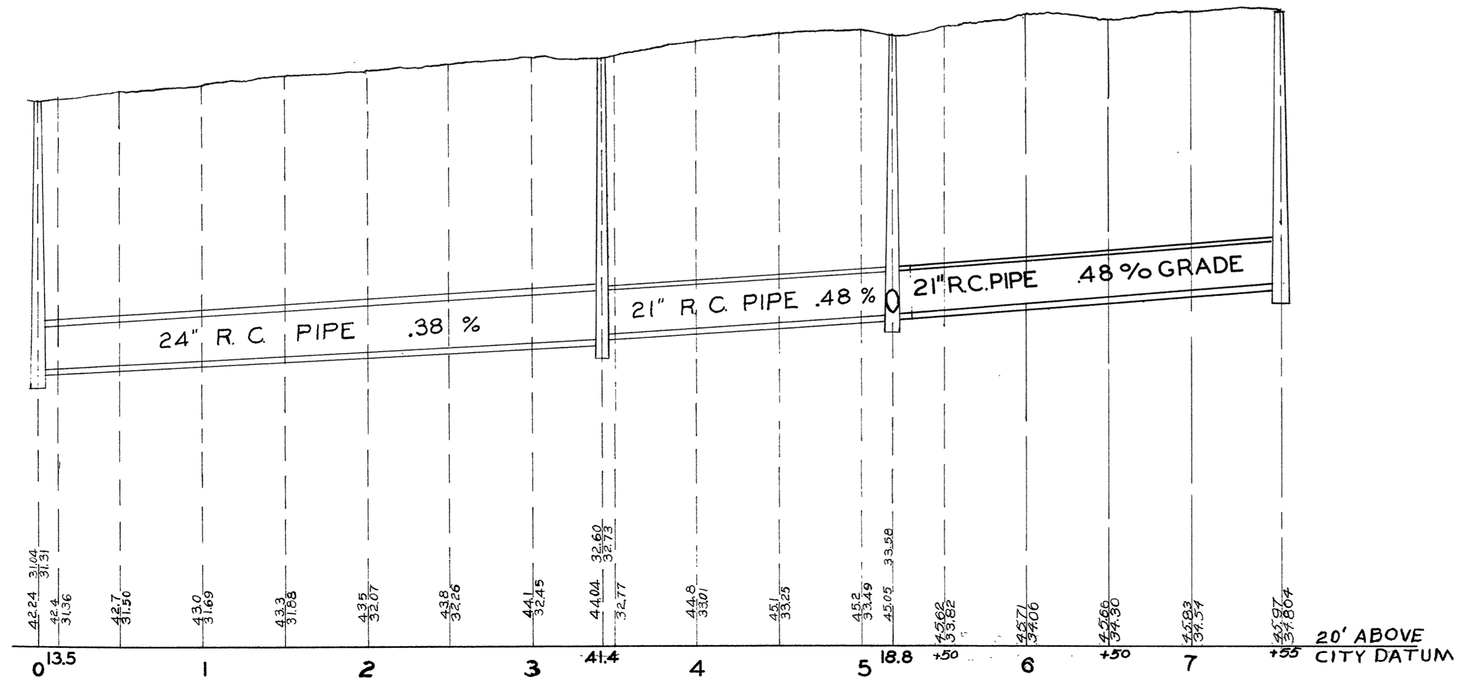
PLAN & PROFILE OF SEWER ON 22 ND AVE. E. FROM E. 13 TH ST. TO ALLEY BET. E. 14 TH & 15 TH ST. THEN TOWARD 23 RD AVE. E.
