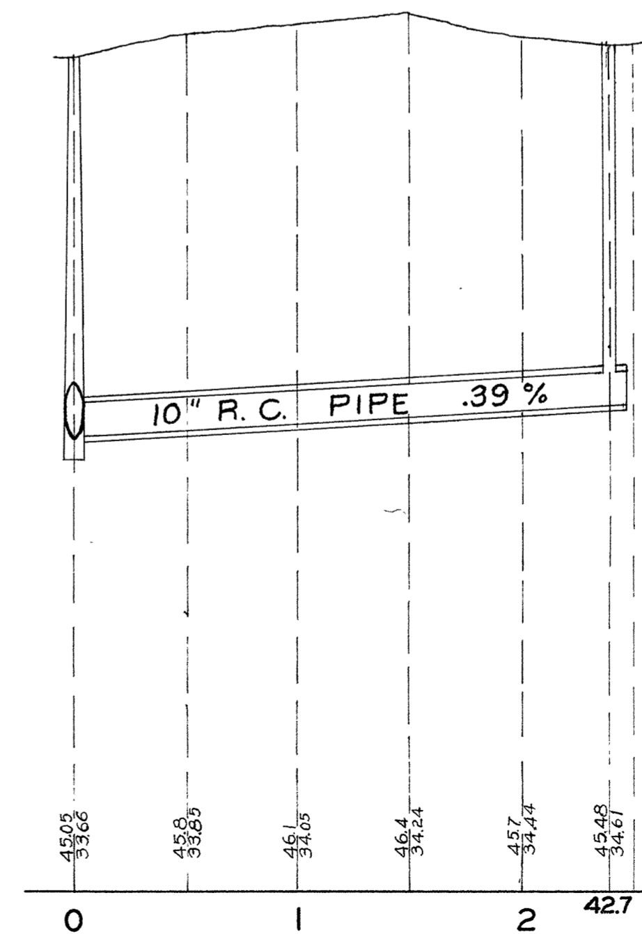
PLAN & PROFILE OF SEWER ON 22 ND AVE. E. FROM E. 13 TH ST. TO ALLEY BET. E. 14 TH & 15 TH ST. THEN TOWARD 23 RD AVE. E.
