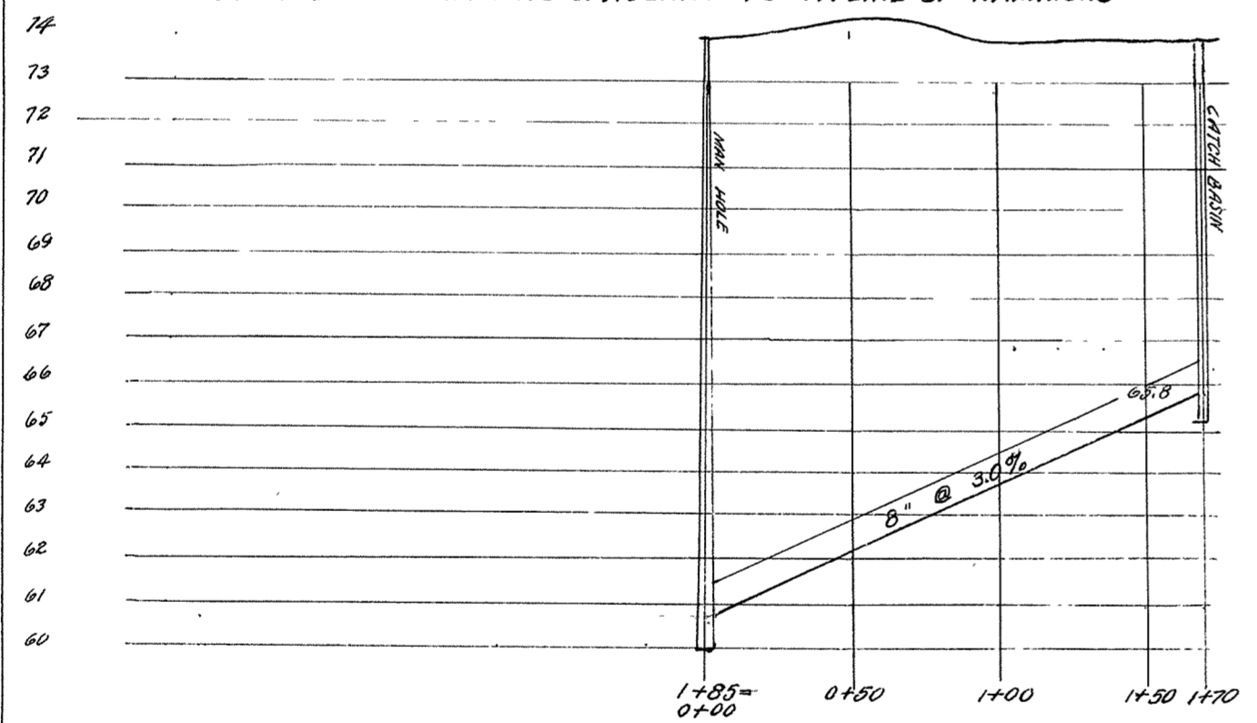
LATERAL SEWER IN ALLEY N. OF 58 TH ST., FROM ALLEY BET. HAMMOND & HUGHITT TO W. LINE OF HAMMOND
