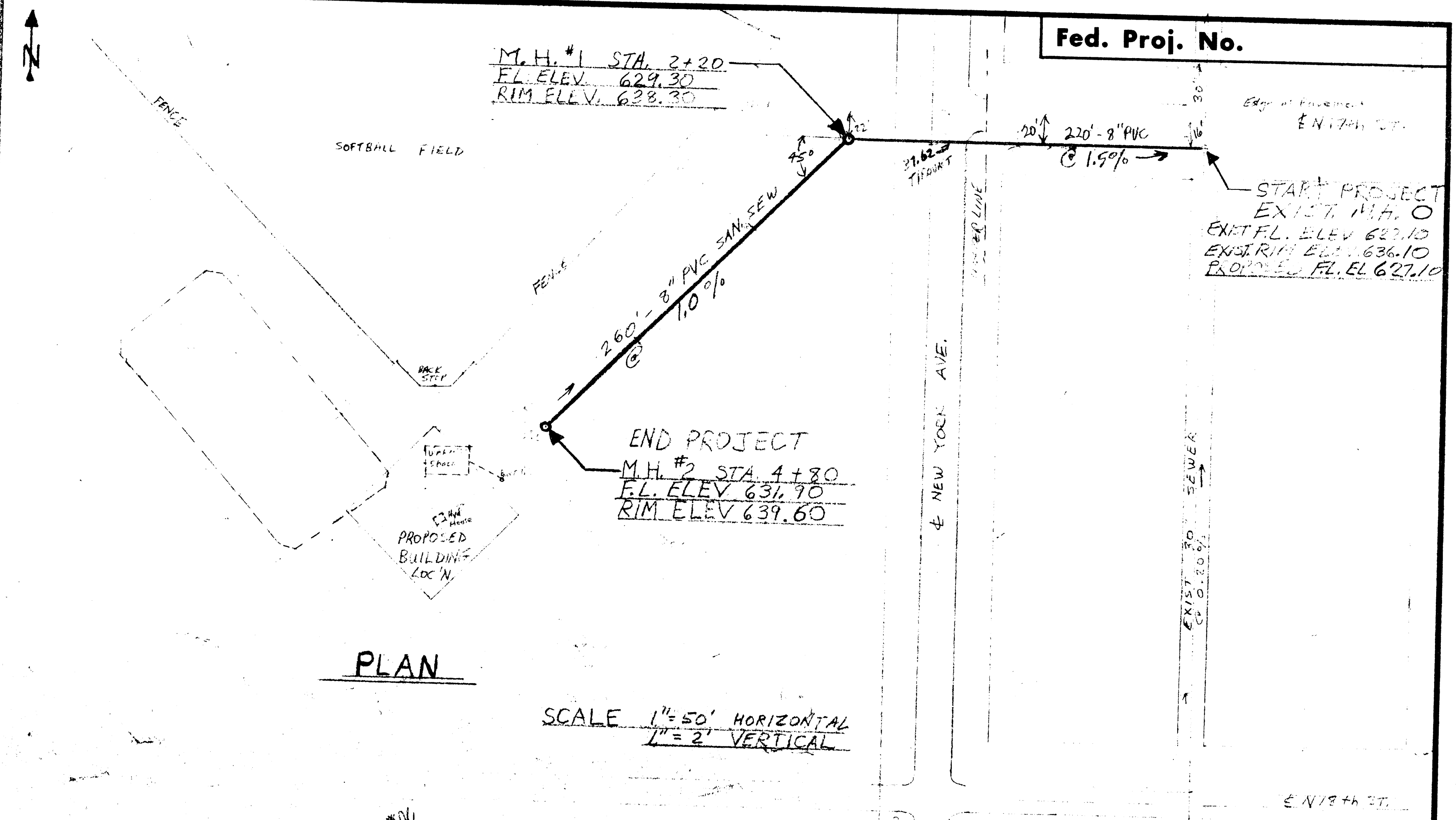
PROPOSED DROP MANHOLE AT EXIST. MANHOLE 0 STA. 0+00
