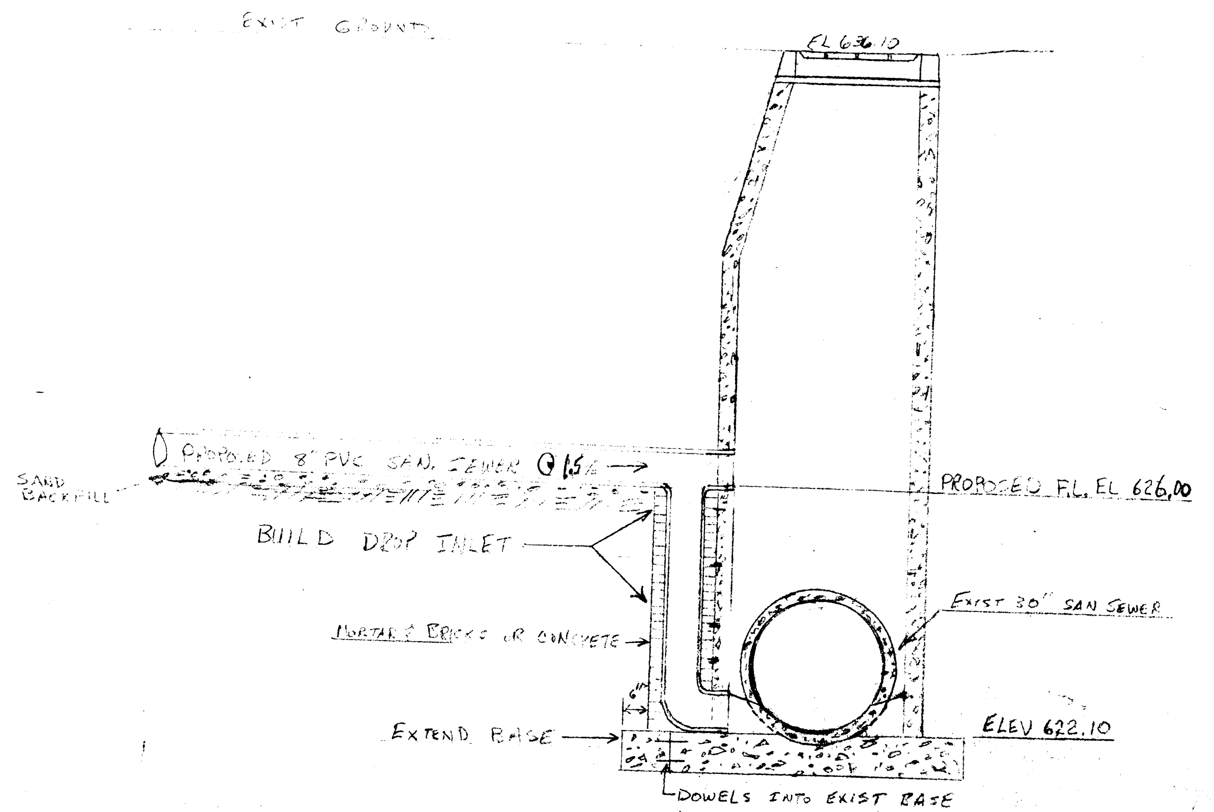
PROPOSED DROP MANHOLE AT EXIST. MANHOLE 0 STA. 0+00
