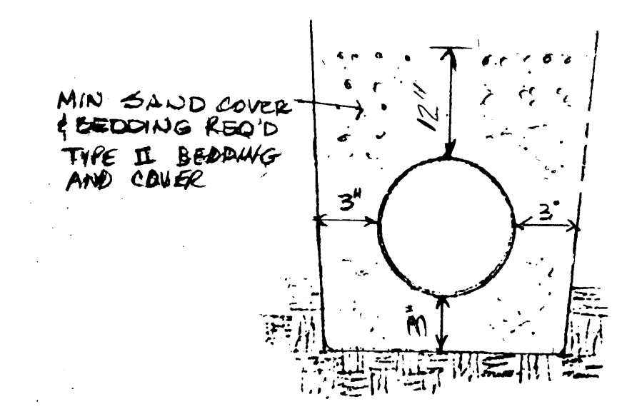
TRENCH BACKFILL DETAIL
