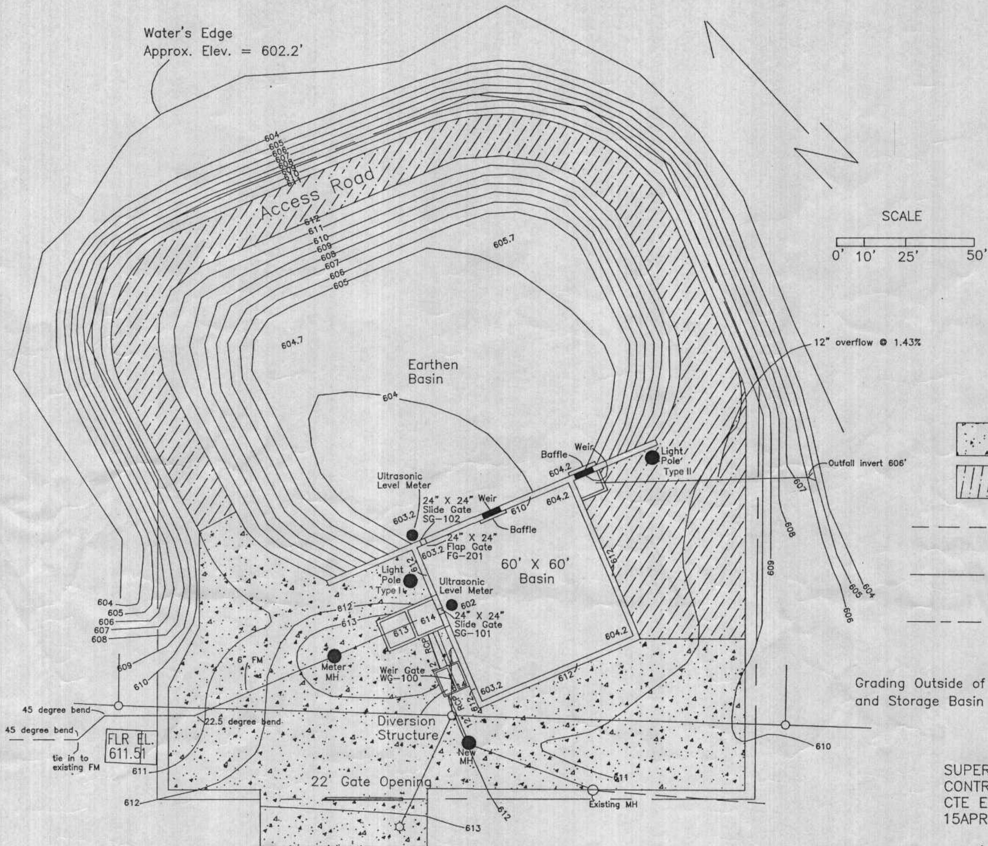
LS 7 SITE PLAN (REVISED)
