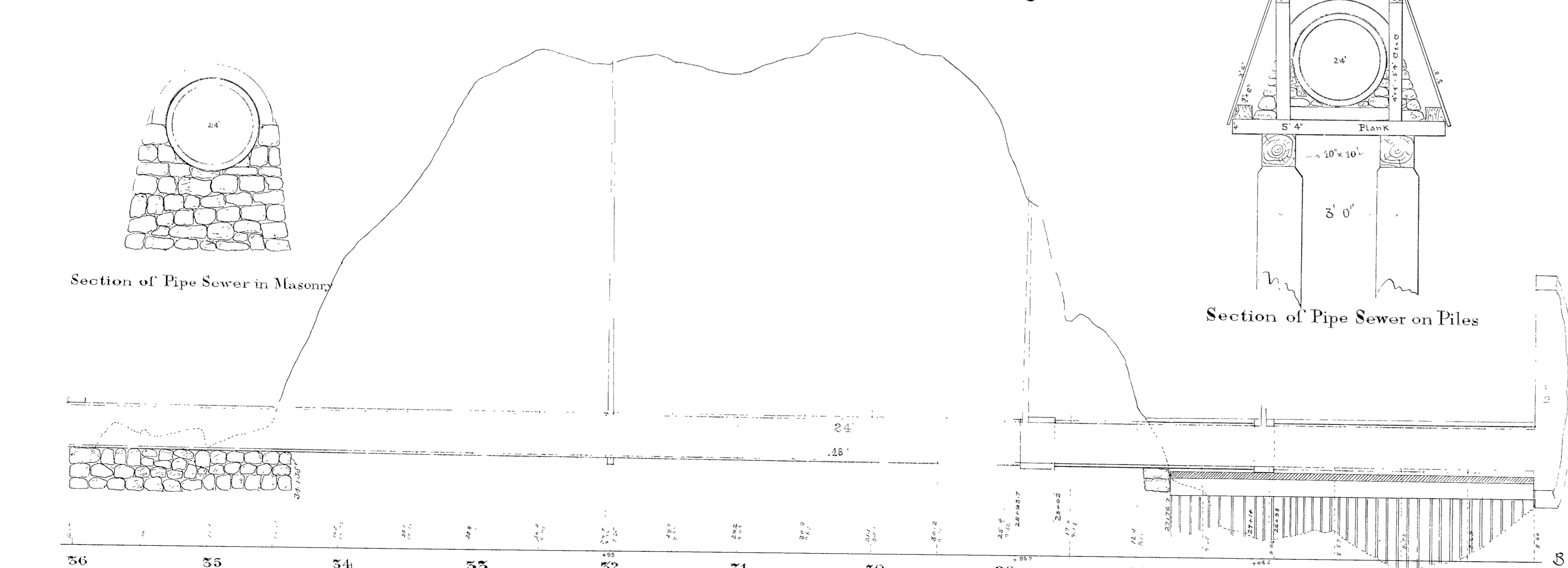
Profile and Plan of Sewer in K St. and Laurel Ave. from Alley between W. 8th & W. 9th Sts. to Hill Ave.
