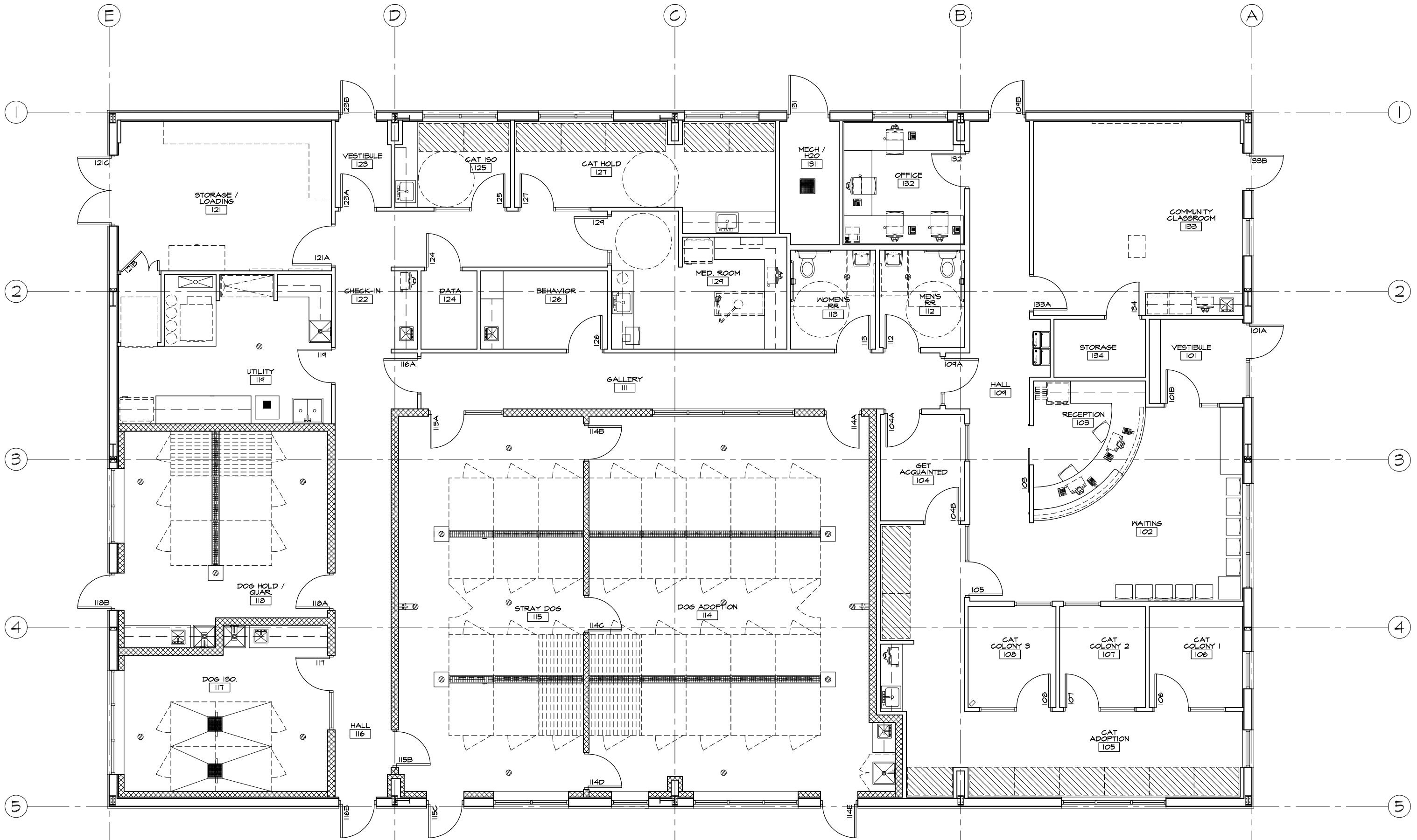
1 SUPERIOR ANIMAL SHELTER - FLOOR PLAN SCALE: 1/8" = 1'-0"
