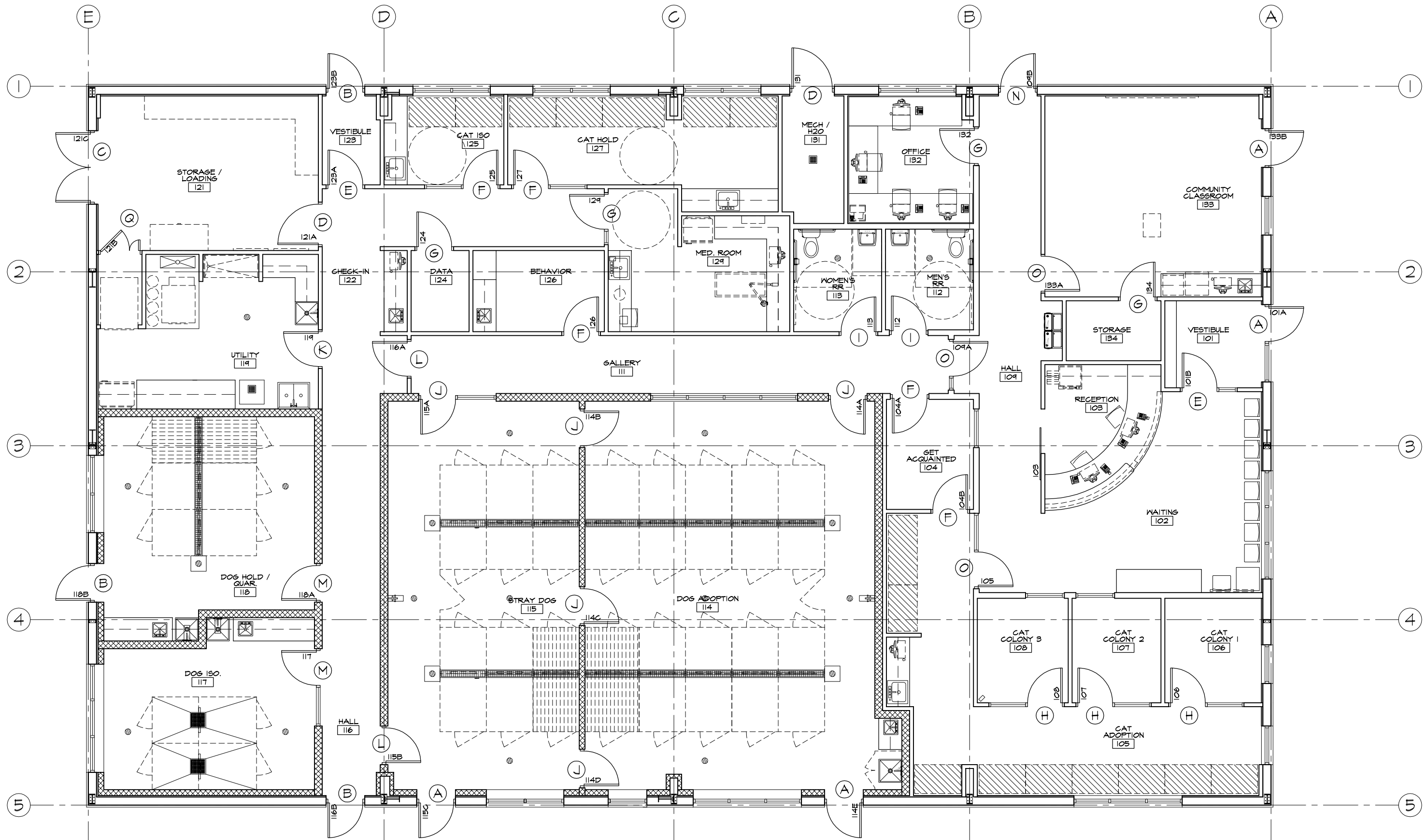
1 SUPERIOR ANIMAL SHELTER - DOOR HARDWARE DIAGRAM SCALE: 1/8" = 1'-0"
